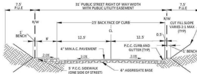
31' R.O.W LOCAL STREET NO PARKING
