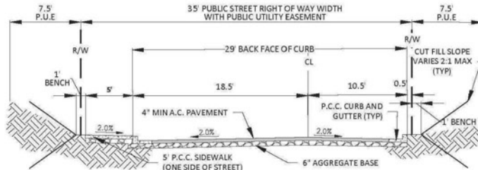
35' R.O.W LOCAL STREET PARKING ONE SIDE
